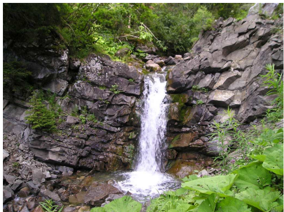
Figure 67. Rio Cordon stream, lower reaches: morphological channel bed characteristics
