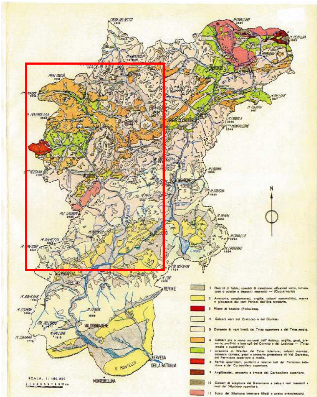
Figure 12: schematic geologic map of the Piave river basin.
