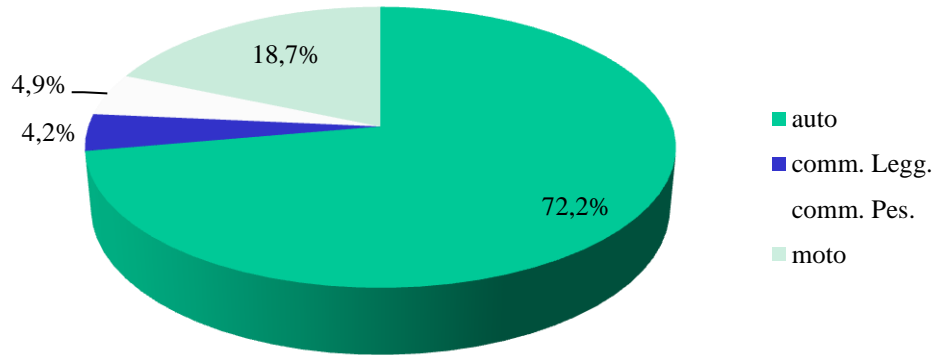
CO (%)
