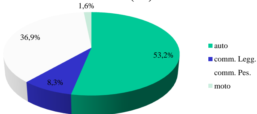
PM10 (%)
